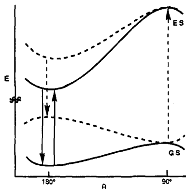
Figure 1. Potential energy diagrams for absorption and emission of diketones as a function of the dihedral angle \theta for rotation around the OC-CO bond: (—) anti coplanar ground state; (---) twisted ground state. A common energy for the 90° geometry, with zero conjugative stabilization and zero steric destabilization, is assumed.
